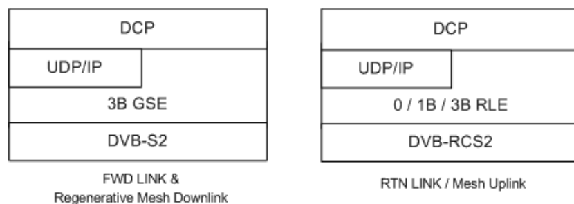
Figure D.1: DCP FWD/RTN protocol stacks
