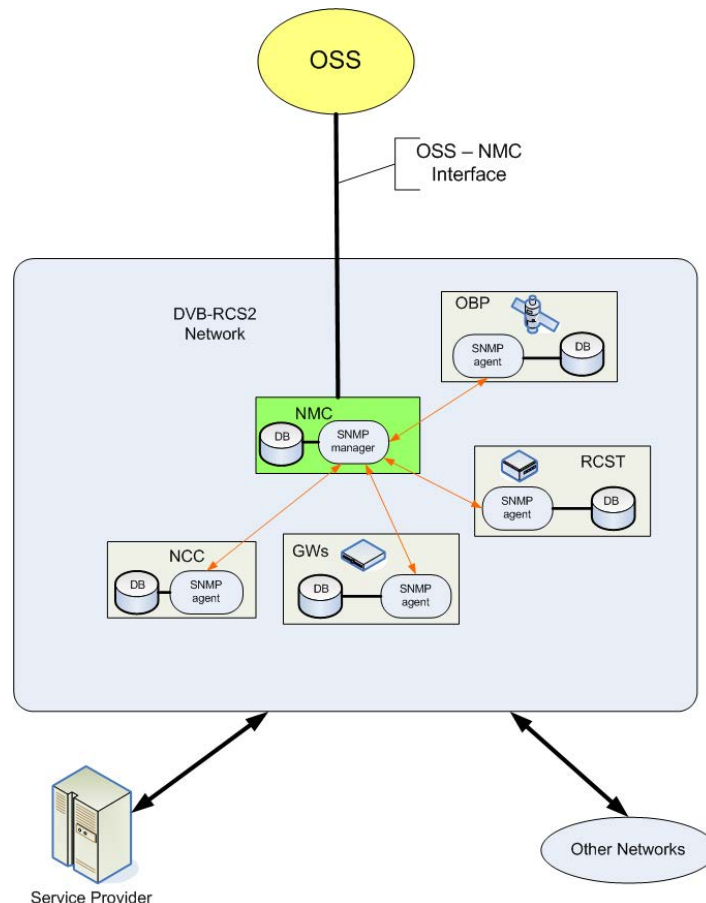
Figure 8.1: Management Reference Architecture
