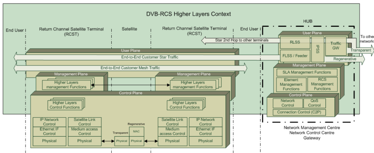
Figure 4.3: Elements functional architecture mapped in user, control and management planes
