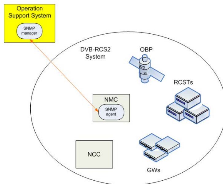
Figure 8.5: OSS-NMC management architecture
