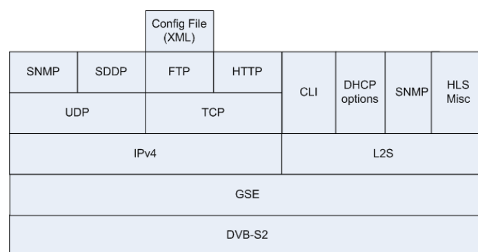
Figure 8.7: Protocol Stack for RCST satellite interface management (return link)
