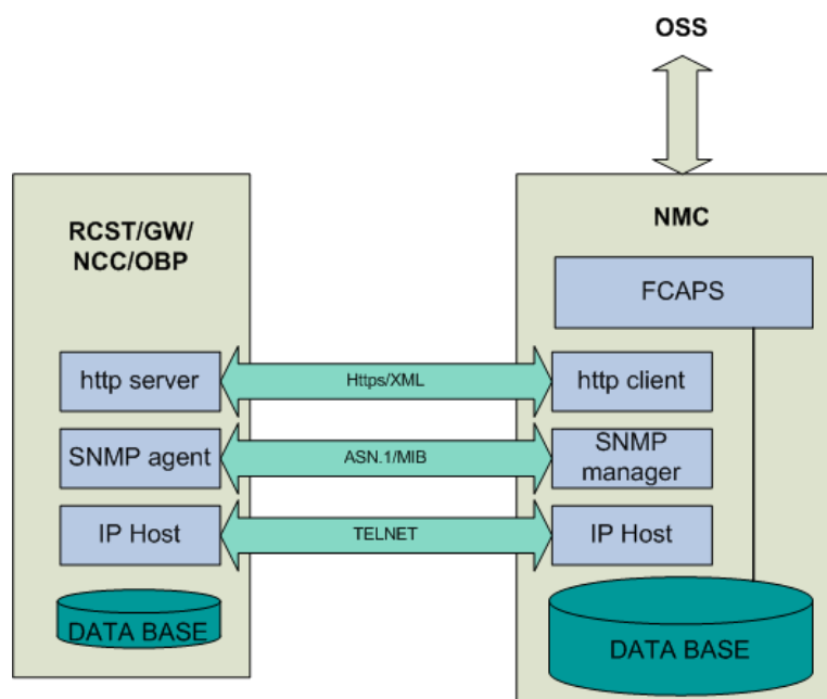
Figure 8.2: RCST - NMC management interactions
