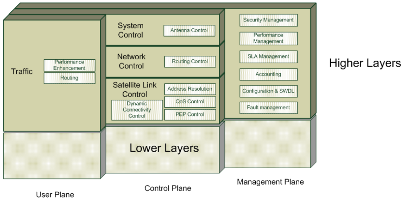
Figure 4.2: Higher layers functional modules
