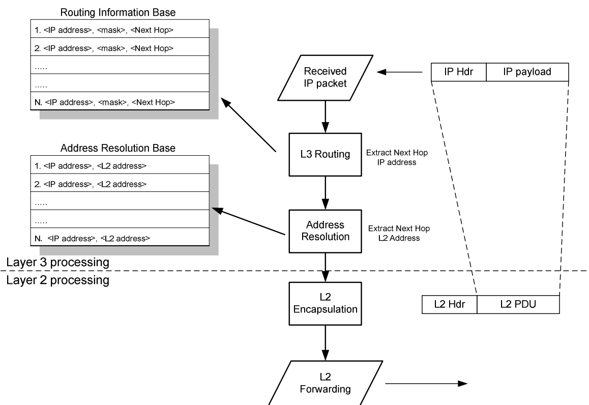
Figure 7.1: RCST Unicast IP packet forwarding
