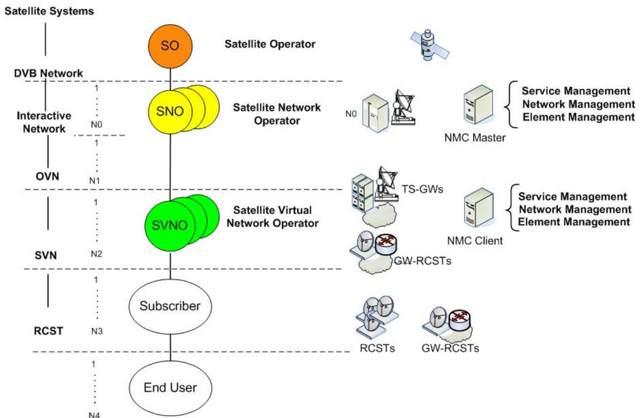
Figure 4.1: DVB-RCS2 actors and roles
