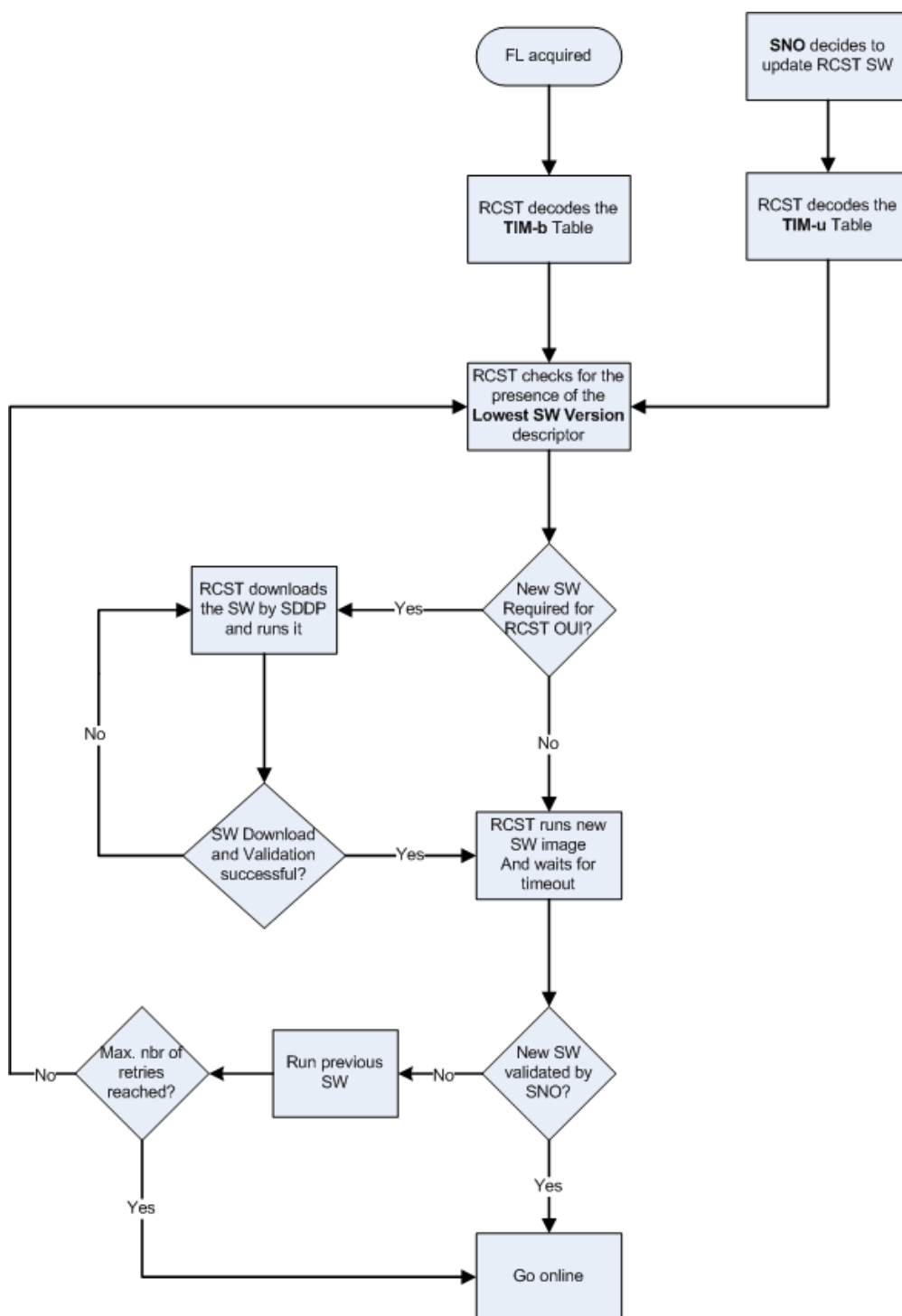
Figure 8.9: RCST SW check and download
