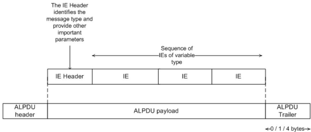
Figure D.2: DCP messages structure over L2
