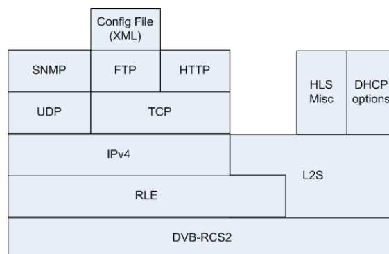
Figure 8.7: Protocol Stack for RCST satellite interface management (return link)
