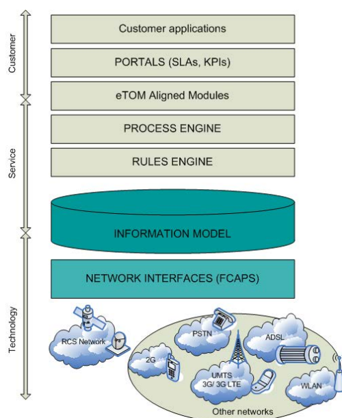
Figure 8.4: OSS-NMC management Interface
