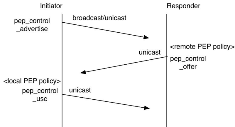
Figure 9.2: PEP Negotiation Exchange
