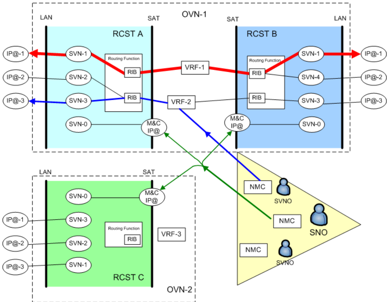
Figure 7.4: OVN, SVN, and VRF domains
